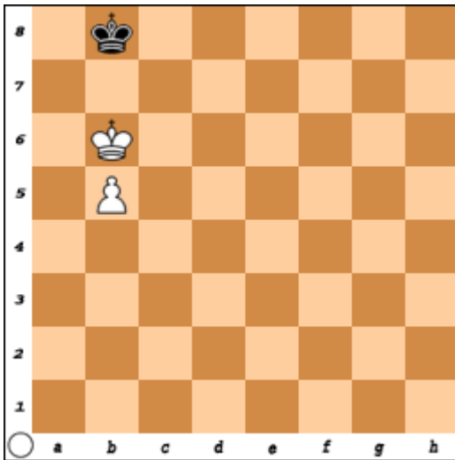
Stelling na 61.Kb6 (analyse)
